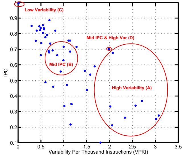
(b) Variability & IPC
