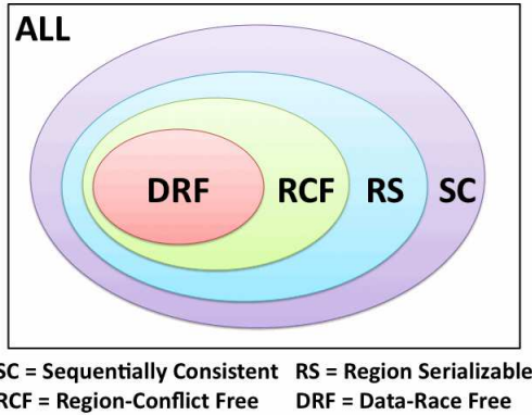
Figure 2. The relationships among various properties of a program execution.
