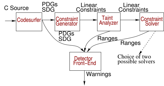
Figure 1: Overall Architecture of the Buffer Overrun Tool
