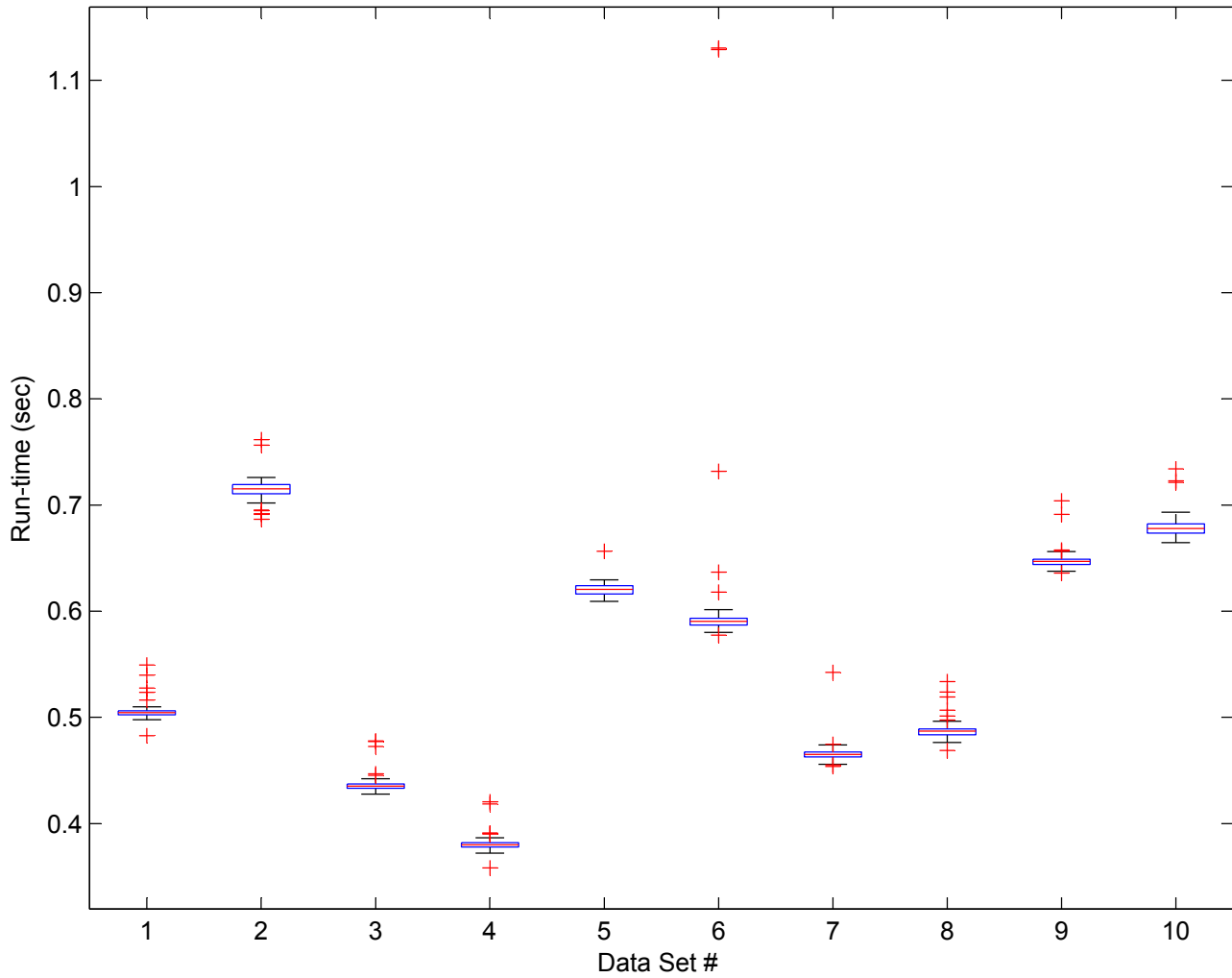
SQRS Algorithm Average (100x) Runtimes for 10 ECG Data Sets
