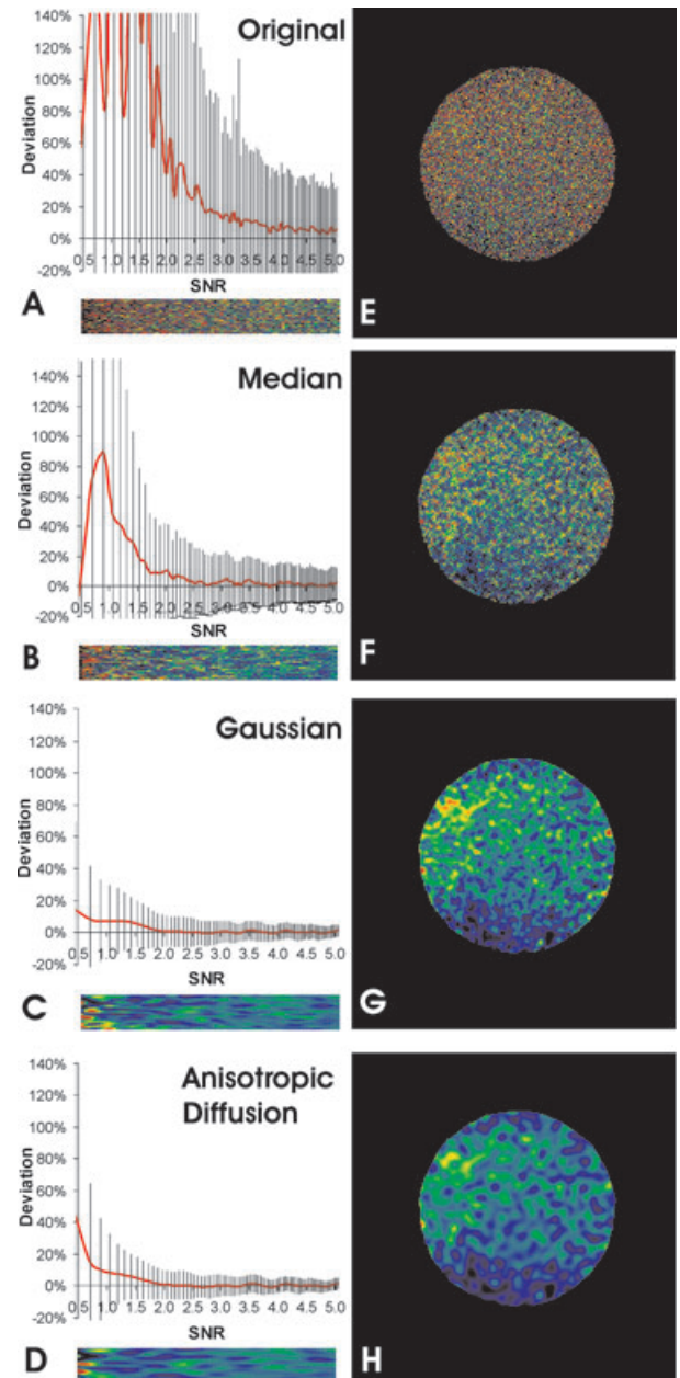
Fig. 4. Restoration of ratio images with conventional noise reduction filters. Noisy grey scale (A–D) or bead images (SNR of denominator image about 2.6 before noise reduction; E–H) are shown without denoising (A, E), or after noise reduction with a median filter (B, F), Gaussian filter (C, G), or anisotropic diffusion filter (D, H) before taking the ratio. Systematic error relative to the correct value is calculated for the grey-scale images as a function of initial SNR between 0.5 and 5.0 (A–D plots). Vertical lines indicate the standard deviation. The corresponding ratio image is rendered in pseudo-colour and enlarged horizontally to match the scale shown in the graph. Pseudo-colour rendering is performed according to the colour scale shown in Fig. 3. Note the dramatic restoration of average intensity ratios towards correct values, which should be blue–green in pseudo-colour for both types of images as shown in Fig. 3(A). However, although Gaussian and anisotropic diffusion filters show better restoration of ratio than the median filter, both create artefacts of discrete ratio domains.
