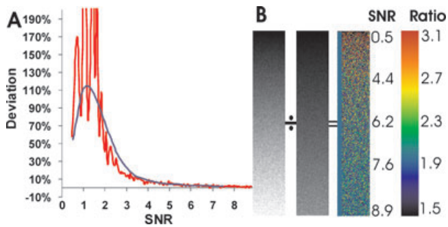
Fig. 2. Estimation of noise-induced systematic error in ratio imaging. Systematic error relative to the correct value is calculated as a function of SNR, assuming a Gaussian noise profile (A, blue curve). A more realistic estimation was obtained by dividing two grey scale images with a constant ratio, with added noise that simulates what was measured from an EMCCD camera (B). SNR (B, numbers under 'SNR') increases with the intensity as expected. The corresponding intensity ratio increases with decreasing intensity or SNR (A, red curve, and B; colour-coding of the ratio indicated in the scale under 'Ratio'), reaching a peak at SNR \sim 1 . The correct ratio ( =2 ) as rendered in pseudo-colour is indicated as the blue bar to the left of the pseudo-colour image.
