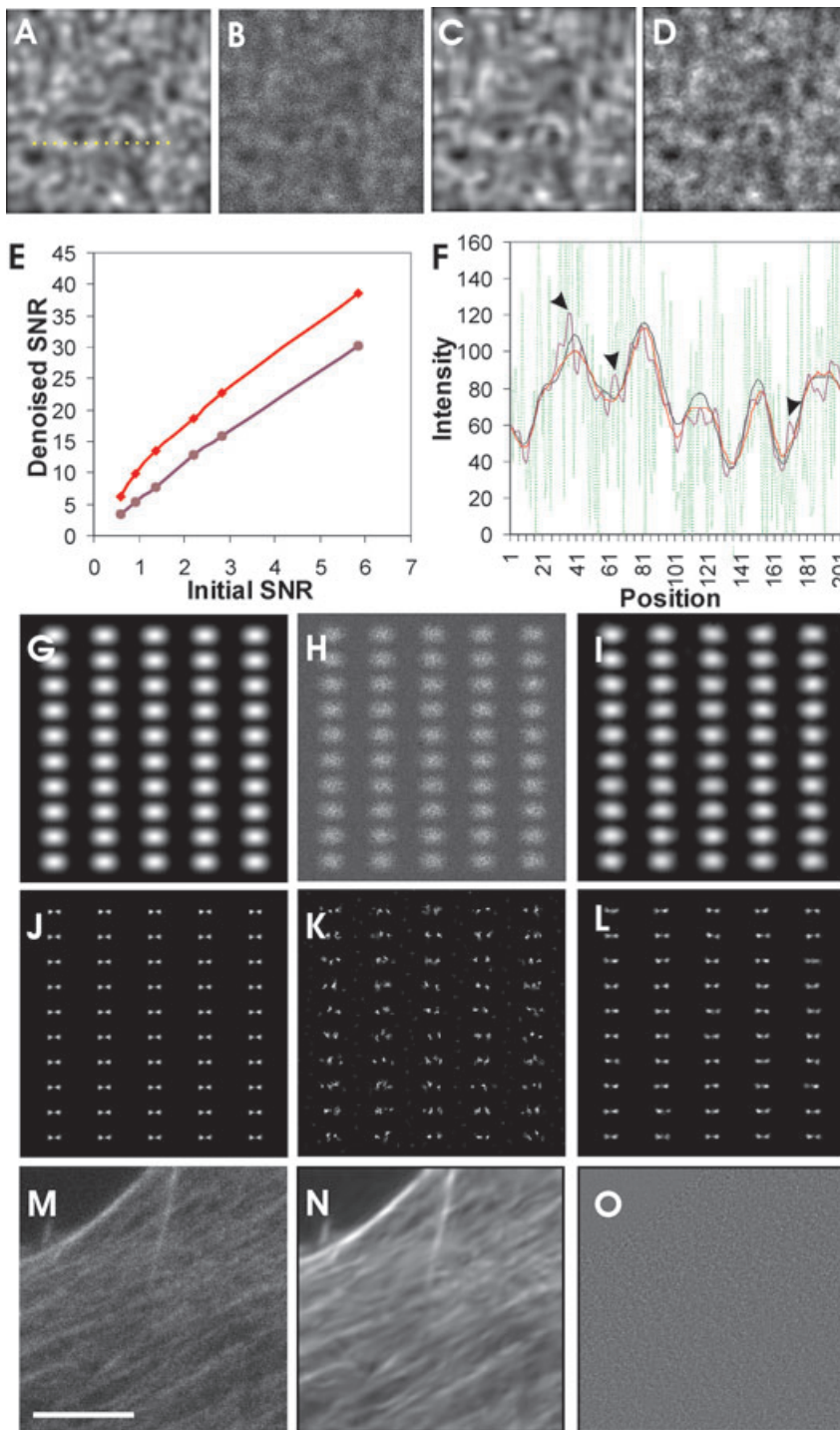
Fig. 5. Denoising with a statistically based multi-resolution filter. The simulated image consists of 2000 zeroth-order Airy disks distributed randomly in an area of 300 \times 300 pixels (A). Noise is added to the image according to the characteristics of an EMCCD camera, creating an image of overall SNR \sim 1.36 (B). The image is then denoised with either a multi-resolution BLS-GSM filter (C) or a Gaussian filter (D). Note the striking restoration of image with the BLS-GSM filter, whereas the Gaussian filter creates numerous granule-like artefacts. SNR increases by a factor of 6.6–10.3 with the BLS-GSM filter (E, red line), and by a factor of 5.2–5.8 with Gaussian filter (E, purple line). Measurement of intensity profile along a line (A, dotted line) shows large fluctuations before denoising (F, green line), relative to the true profile (F, black line). Although both filters suppress intensity fluctuations, the Gaussian filter (F, purple line) generates numerous small peaks not seen in the truth profile (F, arrowheads). The profile after processing with the BLS-GSM filter closely resembles the truth profile, with the intensities agreeing within 10% (F, red versus black lines). Application of the BLS-GSM filter to simulated noisy images of pairs of Airy disks, separated at approximately 0.6 Rayleigh resolution limit, allows the application of two-dimensional deconvolution to resolve the point sources. Noise is added to the original image (G) to generate an image of SNR < 1.0 (H). Deconvolution of both the original and denoised image (I) generated similar pairs of point sources in a regular pattern. Deconvolution of the noisy image generates many extra points and poorly defined point sources (K). The same filter applied to a noisy image of an NIH3T3 cell stained with Alexa-488 phalloidin (M) dramatically restores the image, revealing many details that are originally masked by the noise (N). The difference between the original and denoised images (residual image; O) shows only random noise, indicating that little or no structures have been lost during denoising. Bar, 5 \mu\text{m} .
