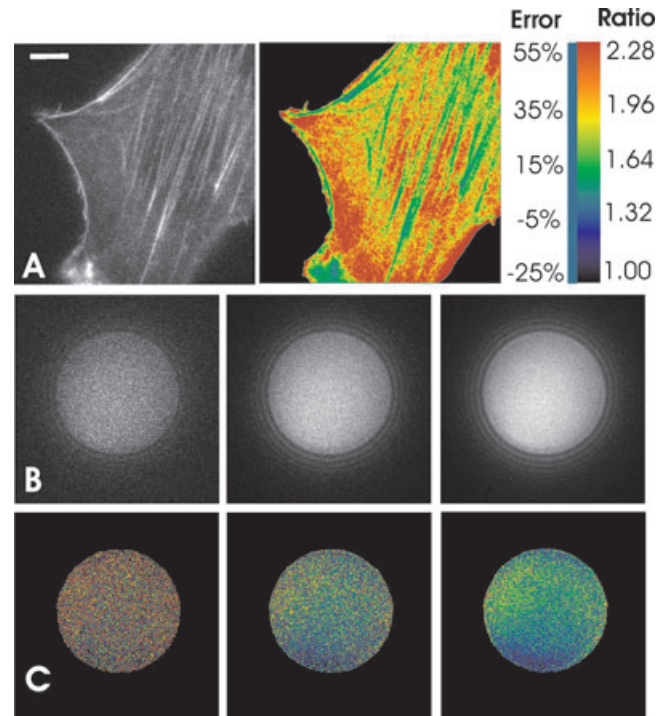
Fig. 3. Noise-induced systematic error in fluorescence ratio imaging. Image of an NIH3T3 cell stained with Alexa-488 phalloidin is acquired at an overall SNR \sim 2.2 (A, left panel). Systematic error at each pixel, if this image were used as the denominator image in ratio imaging, is calculated according to the estimated local SNR and the theoretical curve shown in Fig. 2(A), and rendered in pseudo-colour (A, right panel). Colour-coding of the relative error is indicated in the colour scale (numbers under 'Error'). The blue bar to the left of the scale indicates the colour for 0% error. Bar, 5 \mu\text{m} . The effect of noise in actual ratio imaging is demonstrated by taking the ratio between images of a 5.68- \mu\text{m} polychromatic bead acquired with a GFP (numerator image; not shown) or a YFP (denominator image; B) filter set. The YFP images have an SNR of 2.6 (left), 6.1 (middle), and 11 (right), respectively, in the bead area. Ratio image is rendered in pseudo-colour (C), as indicated in the colour scale (numbers under 'Ratio').
