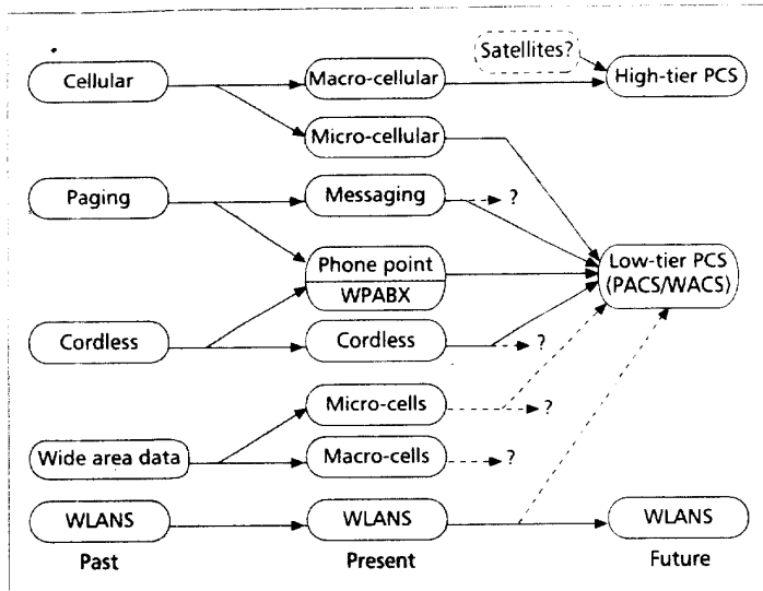
■ Figure 1. Digital wireless access systems evolution.
