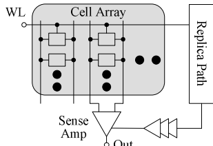
Figure 4. Simplified circuit schematic of an SRAM read path
