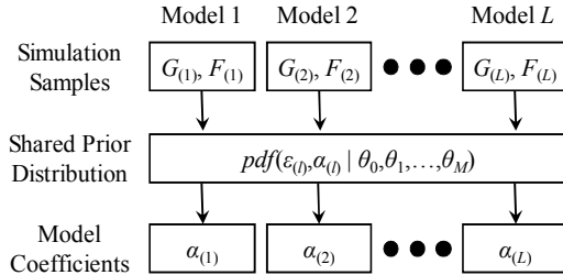
Figure 1. The same prior distribution (i.e., model template) is shared by all performance models for multi-mode/multi-corner sparse regression (MSR).
