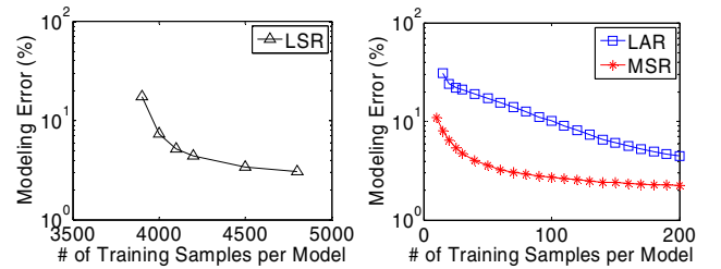
Figure 3. Linear performance modeling error
