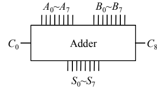
Figure 2. Block diagram of an 8-bit adder
