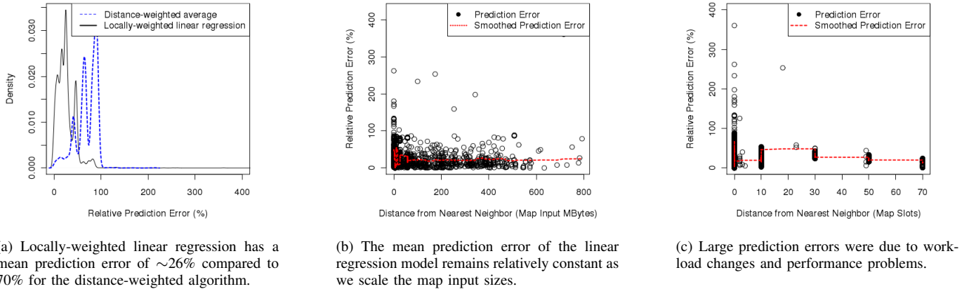
Fig. 8. Trends in the relative prediction error as we scale the map input sizes of three frequently-run jobs.
