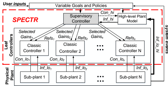
Figure 9. SPECTR overview.
