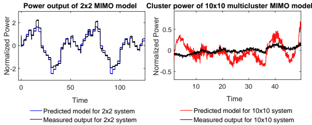
Figure 5. The accuracy of identified system models for a 2 \times 2 MIMO (Figure 2) compared to a 10 \times 10 MIMO (Figure 4). Shown is a single cluster-wide measured output for power, normalized around mean values.
