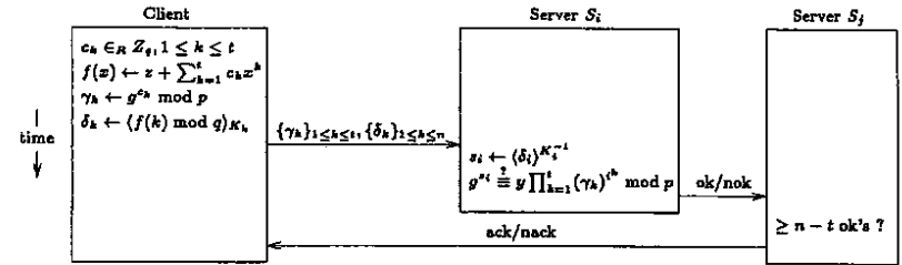
Fig. 3. ElGamal key escrow.
