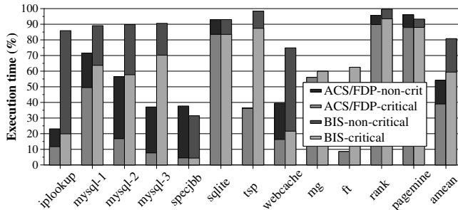
Figure 10. Bottleneck identification on and off the critical path.
