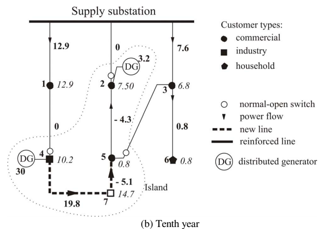
Fig. 5. Optimal Solution for 10 Years Planning Period – Distribution Generator can not be Controlled
