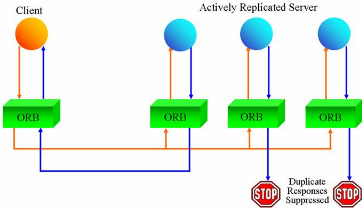
Figure 1 – Active Replication
