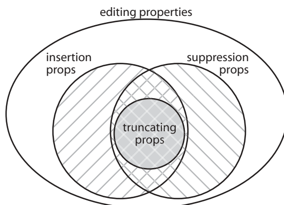
Fig. 4 A taxonomy of effectively enforceable security properties on both uniform and nonuniform systems.
