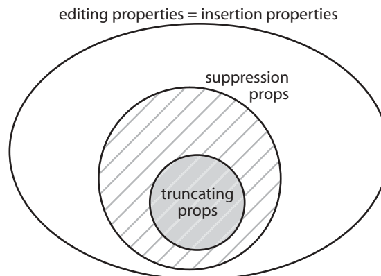
Fig. 3 A taxonomy of precisely enforceable security properties on nonuniform systems.
