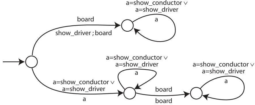
Fig. 1 An insertion automaton that effectively enforces the cable-car policy on a uniform system.
