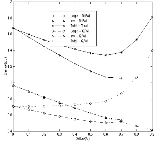
Figure 2. Energy Reduction with voltage scaling. (Delta V = VSS_{INV} - VSS_{LOG} = VDD_{INV} - VDD_{LOG} )
