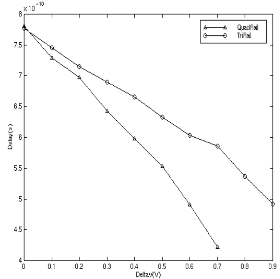
Figure 3. Gate Delay with Voltage Scaling.
