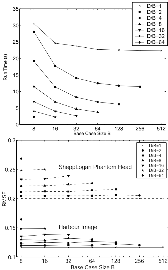
Fig. 3. Runtimes (top) and RMSE (bottom) for different recursion strategies.
