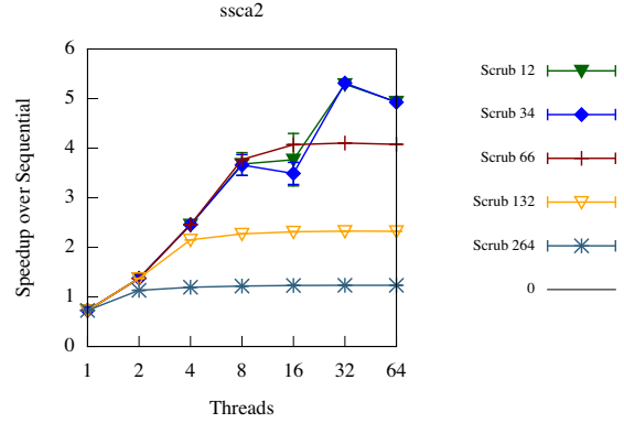
Figure 6: Effect of varying scrub intervals for ssca2 .
