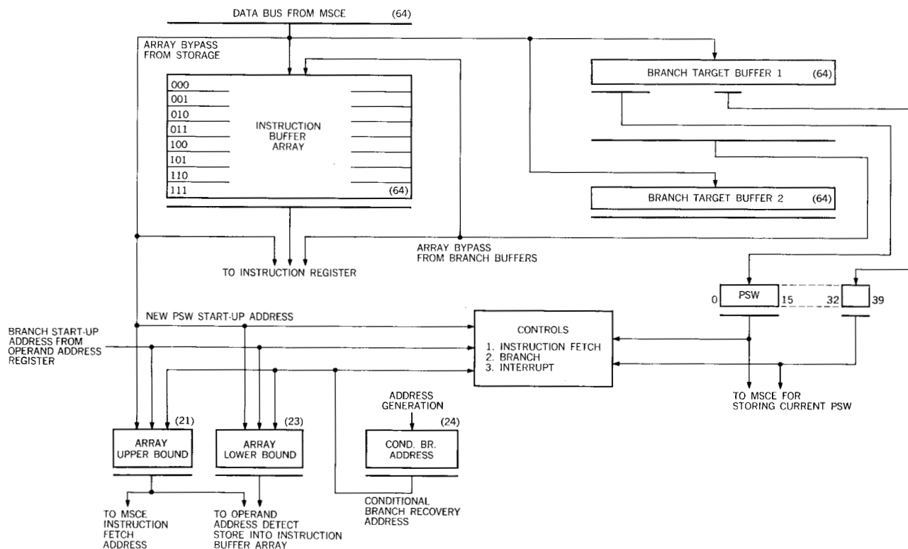
Figure 10 Data paths for the basic instruction supply.
