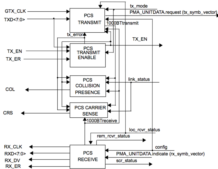
Figure 2.3: PCS Reference Diagram source:802.3z Standard 40.3.1, Figure 40-5 [3]
