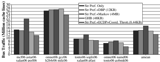
Figure 15. Effect of proposed mechanisms in a four-core system
