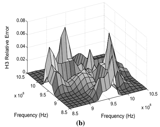
Fig. 8. (a) Original H_3 of the front-end, and (b) relative error of H_3
