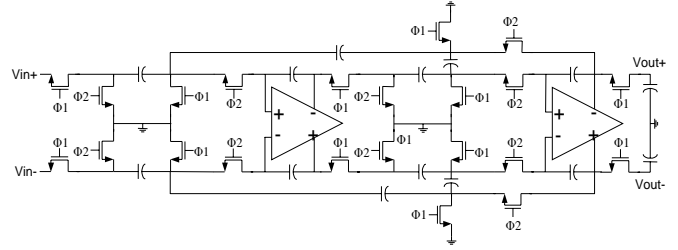
Fig. 4. A switch-capacitor biquad low-pass filter
