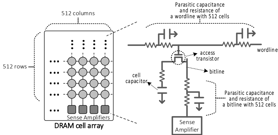
Figure 22: Our SPICE model schematic of a DRAM cell array.
