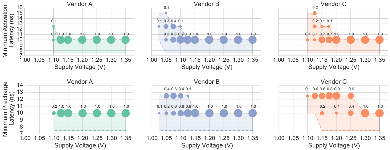
Figure 6: Distribution of minimum reliable latency values as the supply voltage is decreased for 31 DIMMs. The number above each point indicates the fraction of DIMMs that work reliably at the specified voltage and latency. Top row: tRCD_{min} ; Bottom row: tRP_{min} .
