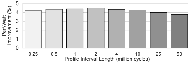
Figure 19: Sensitivity of Voltron’s system energy efficiency improvement to profile interval length.
