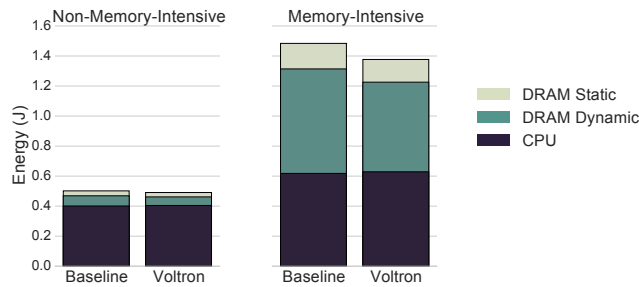
Figure 15: Breakdown of system energy consumption (lower is better).
