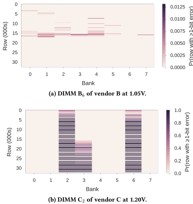
Figure 8: The probability of error occurrence for two representative DIMMs, categorized into different rows and banks, due to reduced voltage.
