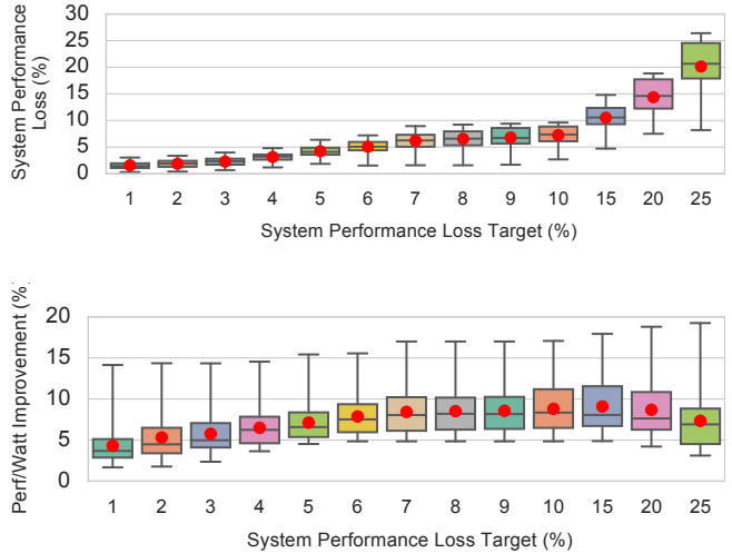
Figure 18: System performance loss and energy efficiency improvement of Voltron as the system performance loss target varies.
