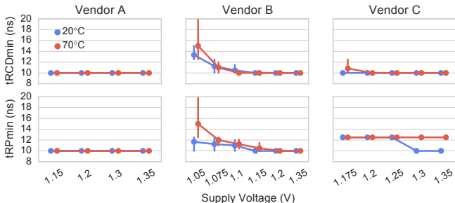
Figure 10: Effect of high ambient temperature (70°C) on minimum reliable operation latency at reduced voltage.
