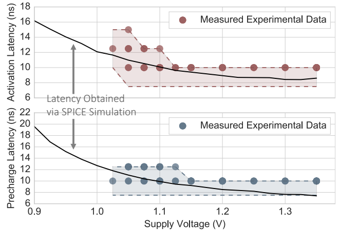
Figure 7: SPICE simulation results compared with experimental measurements from 12 DRAM DIMMs for Vendor B.
