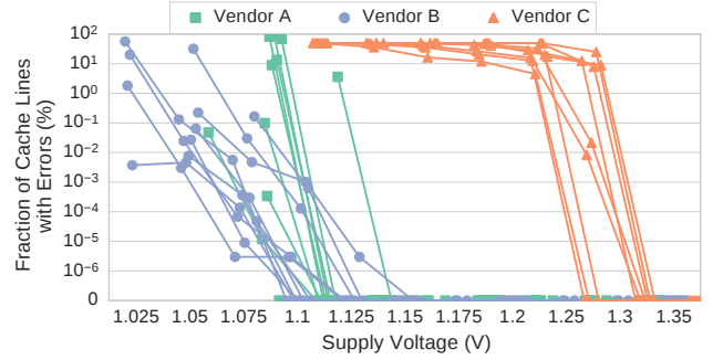
Figure 4: The fraction of erroneous cache lines in each DIMM as we reduce the supply voltage, with a fixed latency.
