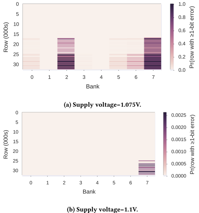
Figure 23: Probability of error occurrence due to reduced-voltage operation in a DIMM from Vendor A.
