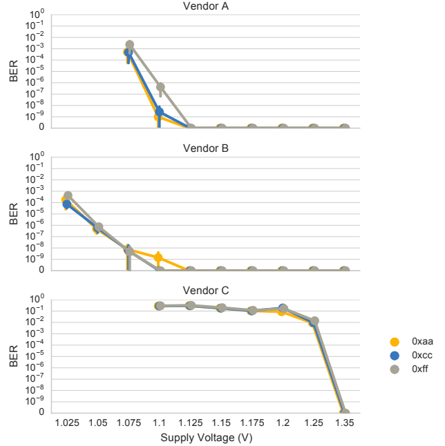
Figure 21: Effect of stored data pattern on bit error rate (BER) across different supply voltage levels.
