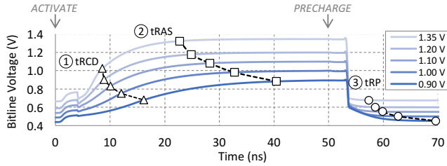
Figure 5: Effect of reduced array supply voltage on activation, restoration, and precharge, from SPICE simulations.
