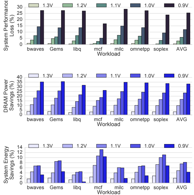
Figure 13: System performance loss and energy savings due to array voltage scaling for memory-intensive workloads.
