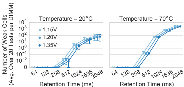
Figure 11: The number of weak cells that experience errors under different retention times as supply voltage varies.
