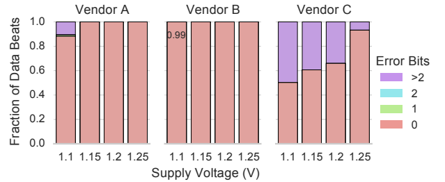
Figure 9: Distribution of bit errors in data beats.
