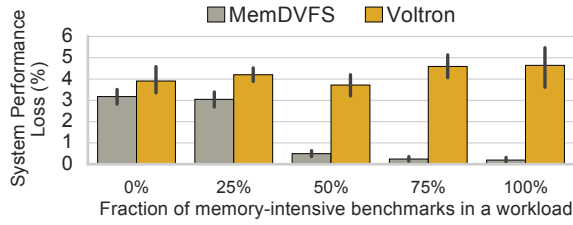
Figure 17: System performance loss and energy efficiency improvement of Voltron and MemDVFS across 50 different heterogeneous workload mixes.
