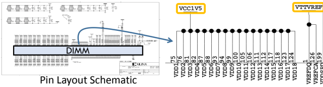
Figure 20: DRAM power pins controlled by the ML605 FPGA board.
