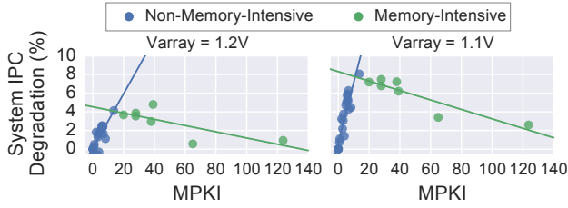
(a) Performance loss vs. last-level cache MPKI.
