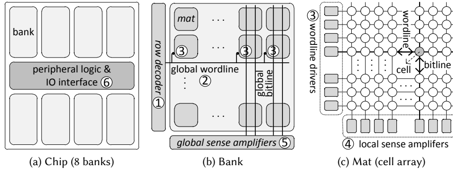
Fig. 2. Hierarchical Organization of a DRAM System
