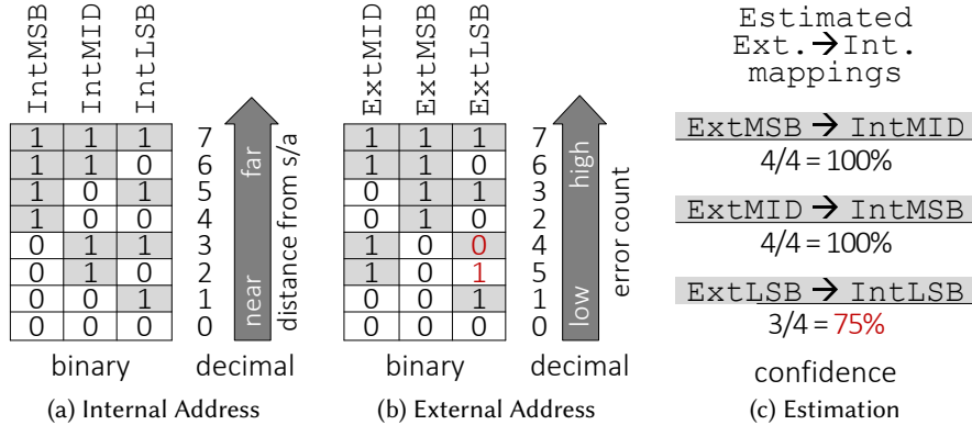
Fig. 10. DRAM-Internal vs. DRAM-External Row Addressing and Estimated Mapping Based on Observed Error Counts for the External Addresses
