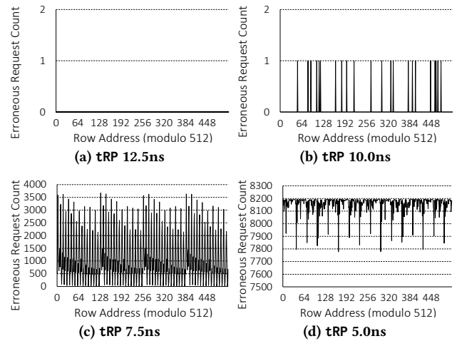
Figure 6: Eroneous Request Count When Sweeping Row Addresses with a Reduced tRP Timing Parameter
