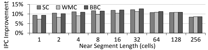
Figure 16. Varying Near Segment Capacity (Inclusive Cache)
