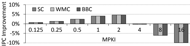
Figure 15. TL-DRAM Performance on Benchmark random
