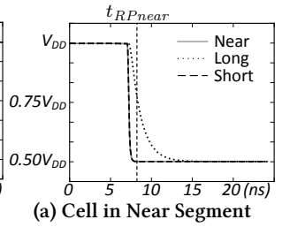
(a) Cell in Near Segment
