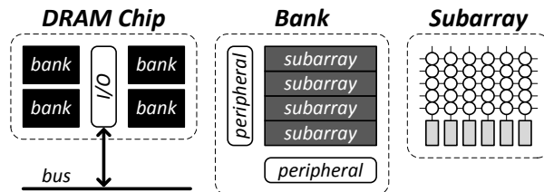
Figure 3. DRAM Organization
