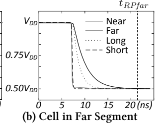
Figure 12. Precharging
