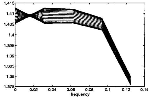
Figure 4: Closeup of ratio of Zak transforms.
