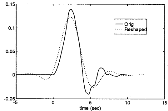
Figure 1: Original D8 and reshaped scaling functions.
