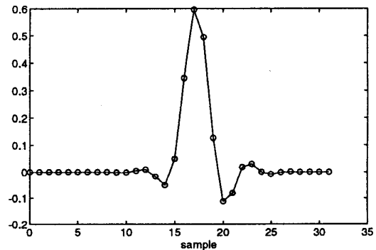
Figure 5: 2-scale coefficients of reshaped D8 signal.
