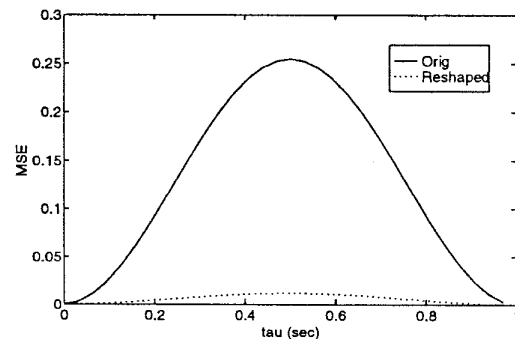
Figure 2: Mean square error \mathcal{E}(\tau) of D8 and reshaped scaling function.
