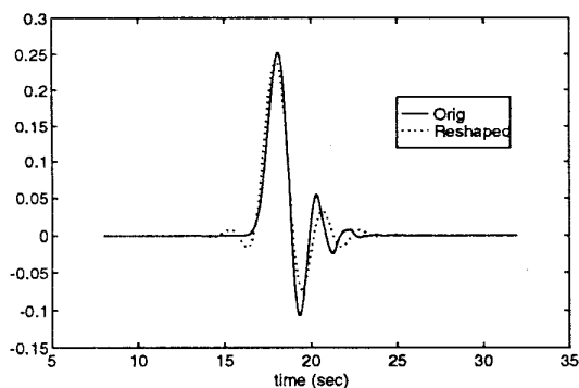
Figure 6: Original D16 and reshaped scaling functions.
