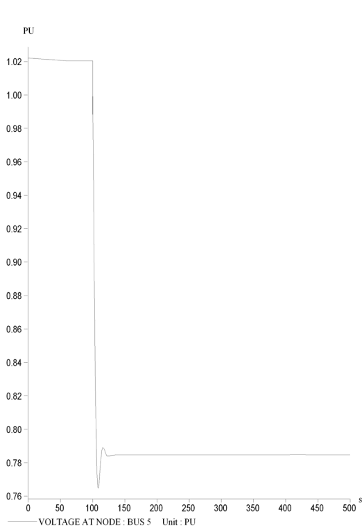
Fig. 4. Voltage change at bus 5 for small load change and high exciter gain
