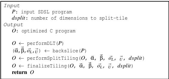
Figure 7: Overview algorithm
