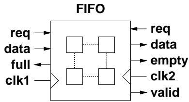
Figure 2. Asynchronous FIFO for interfacing two clock domains
