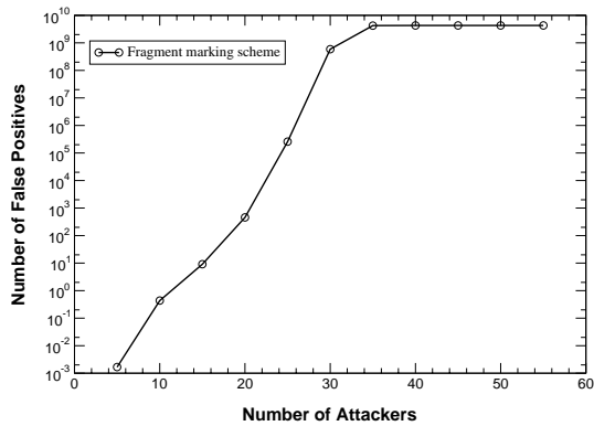
Figure 10: False Positives for FMS
