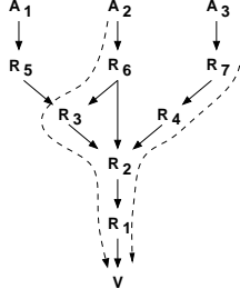
Figure 1: Upstream router map from victim
