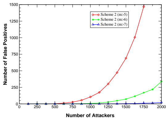
Figure 8: False Positives for Advanced Marking Scheme II
