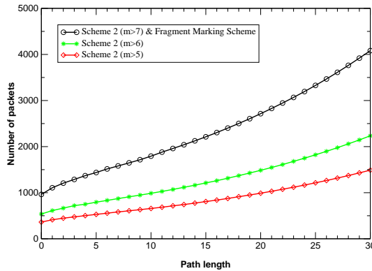
Figure 12: Number of Packets Required for Reconstruction ( q = 4\% )
