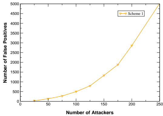
Figure 7: False Positives for Advanced Marking Scheme I
