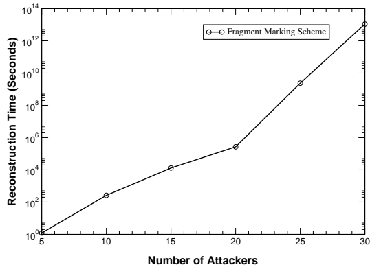
Figure 11: Computation Overhead for FMS
