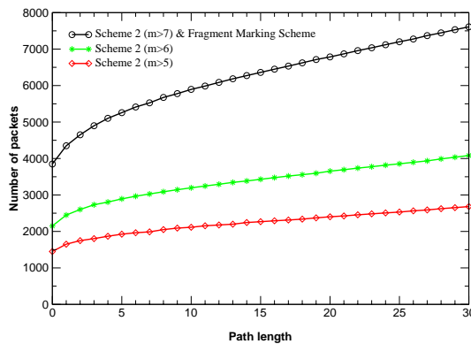
Figure 13: Number of Packets Required for Reconstruction ( q = 1\% )
