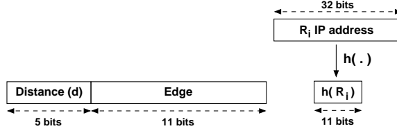
Figure 2: Encoding in Advanced Marking Scheme I
