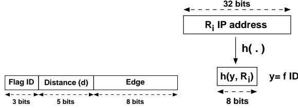
Figure 5: Encoding for Advanced Marking Scheme II
