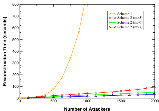
Figure 9: Computation Overhead for Advanced Marking Schemes
